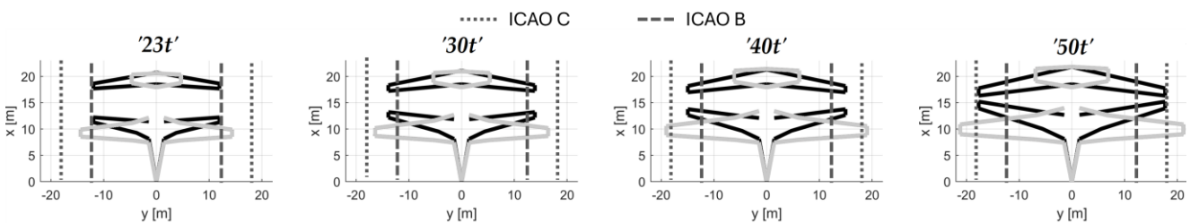
Figure 22. Planform comparison of optimized hybrid-electric configurations; image taken from [83]
