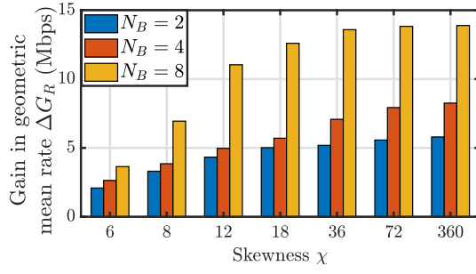
Figure 3: Plot of gain in geometric mean rate \Delta G_R achieved by using k -means clustering over sectoring approach at mmWaves, given P_{limit} = 5 W and N_B = N_B^{k\text{-means}} = N_B^{\text{sector}} .
