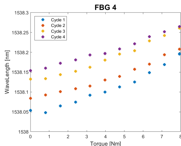
Figure 6 Example of FBG data.
