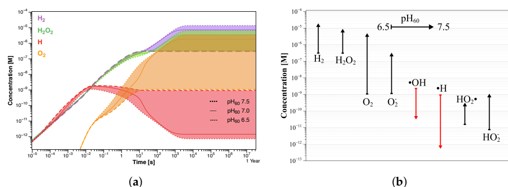
Figure 8. (a) Concentration profiles of the main radiolysis products. The colored regions represent the concentration distributions in the initial pH_{60} range 6.5–7.5. (b) Corresponding concentration trend of the radiolysis products after 1 year of exposure.
