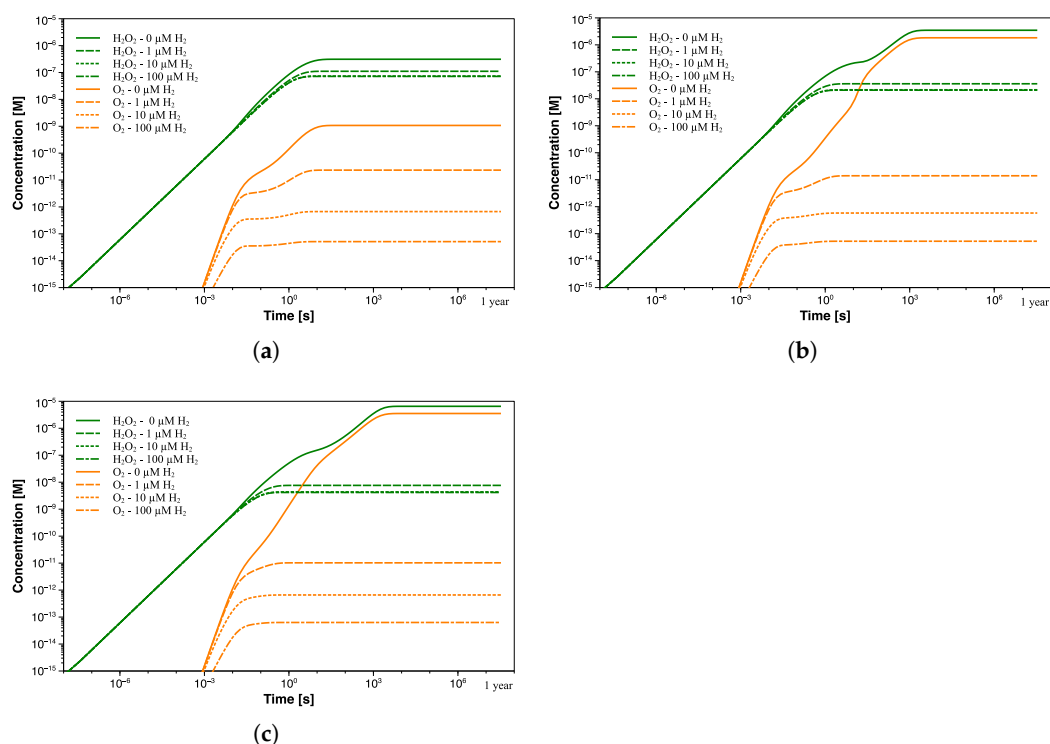
Figure 9. H 2 O 2 and O 2 concentration profiles as a function of exposure time at pH 60 (a) 6.5, (b) 7, and (c) 7.5 with different H 2 concentrations (0–100 \mu M).
