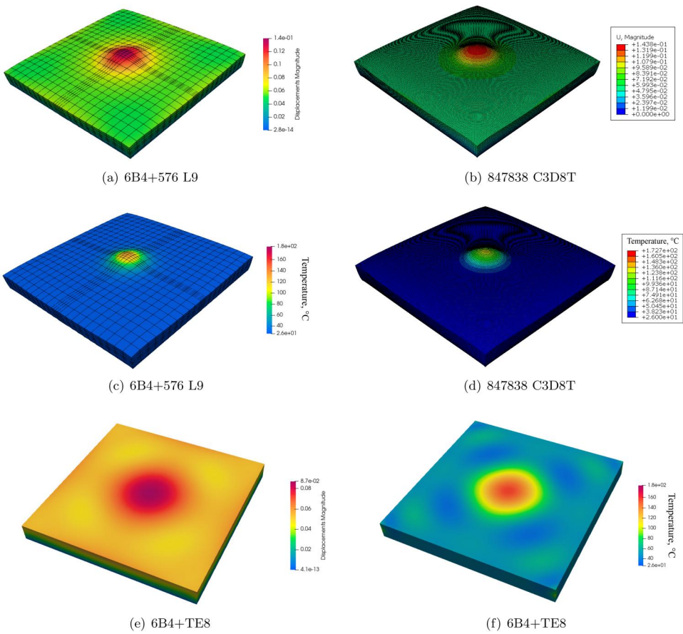
Figure 10. Displacement and temperature contours for the FED with embedded chip. Comparison between the 1D CUF LE9 model (a,c), 3D abaqus (b, d), and TE8 solutions (e, f). The deformations have been magnified by a factor equal to 15.
