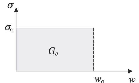
Fig. 2. Dugdale's cohesive law.
