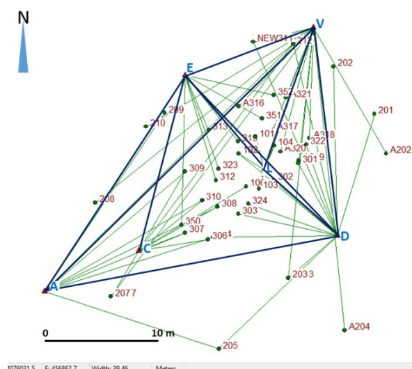
Figure 7. The network (blue) and GCPs (green) topographic schema.
