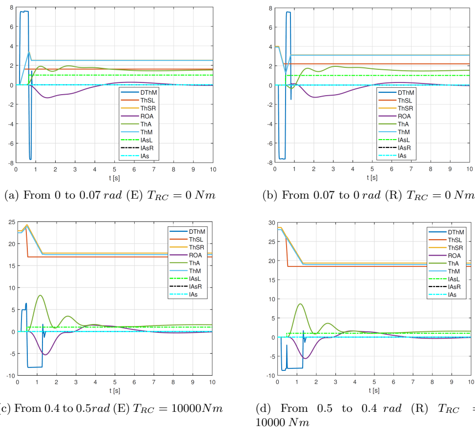
Figure 1: Simulation of nominal (wear-free) flap extraction and retraction in different operational scenarios.
