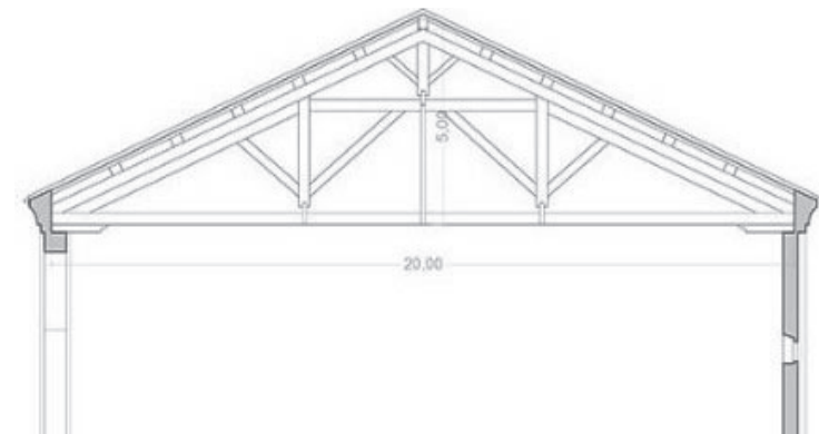
Capriata da https://cjalzumit.wordpress.com/2018/11/24/la-capriata/
