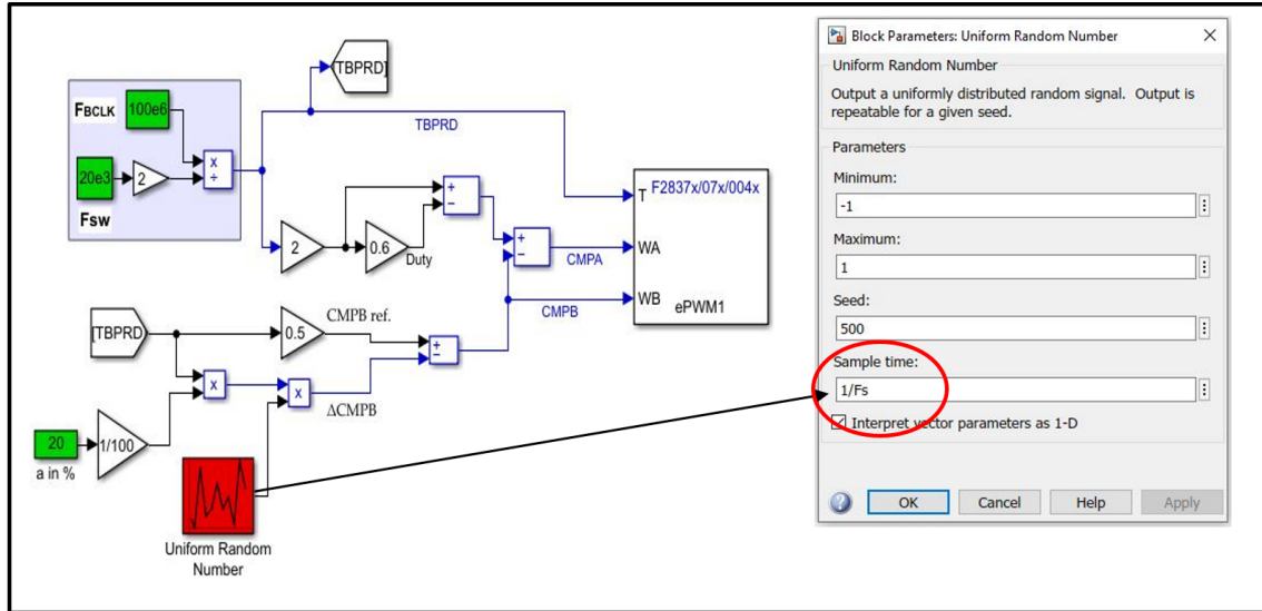
Figure A1. SIMULINK schematics of the implemented RPPM.
