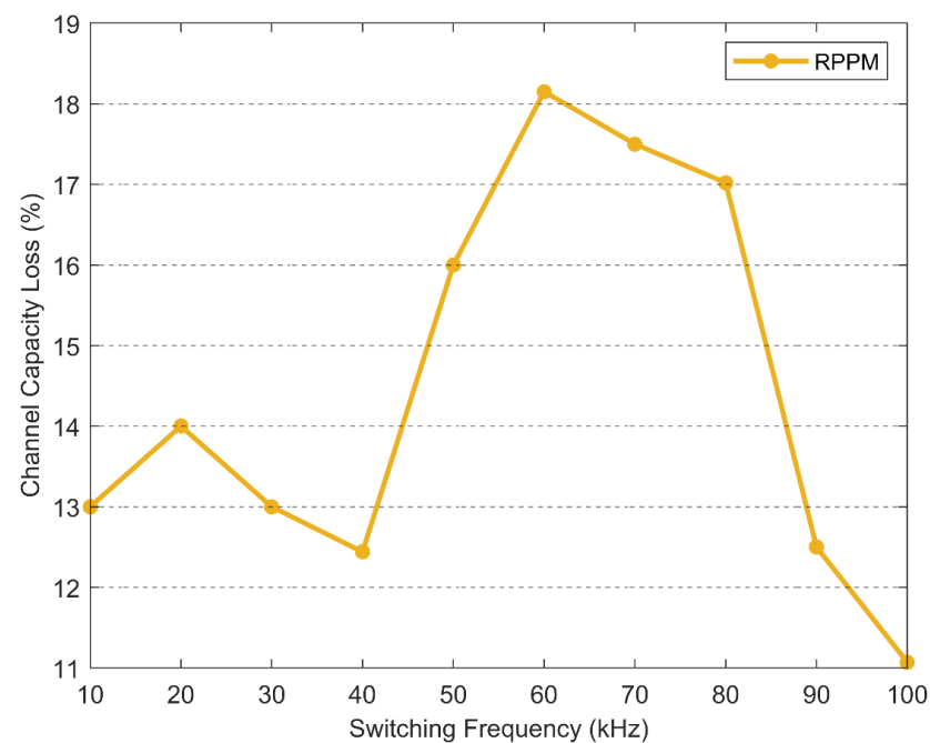
Figure 9. Channel Capacity Loss of the G3-PLC with different switching frequencies applied to the RPPM-modulated DC-DC converter.
