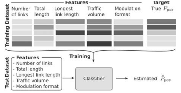
Fig. 1: The classifier structure
