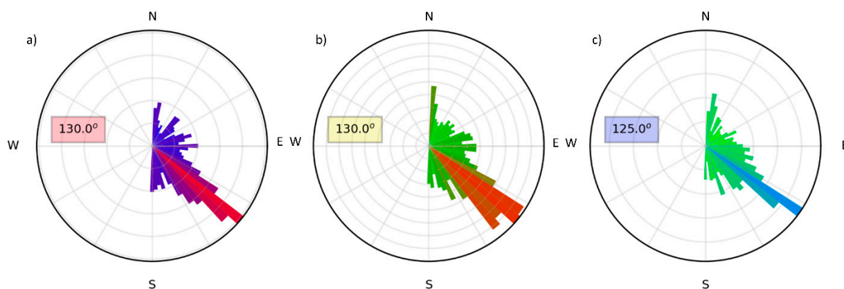
Figure 4. Rose diagrams of the strike direction calculated over the whole period range from (a) the impedance tensor Z , (b) the phase tensor azimuth, and (c) the tipper vector. The color of the bars depends on the number of occurrences in each histogram bin and goes from purple to red for the invariants (a), from green to orange for the phase tensor (b), and from green to blue for the tipper (c).
