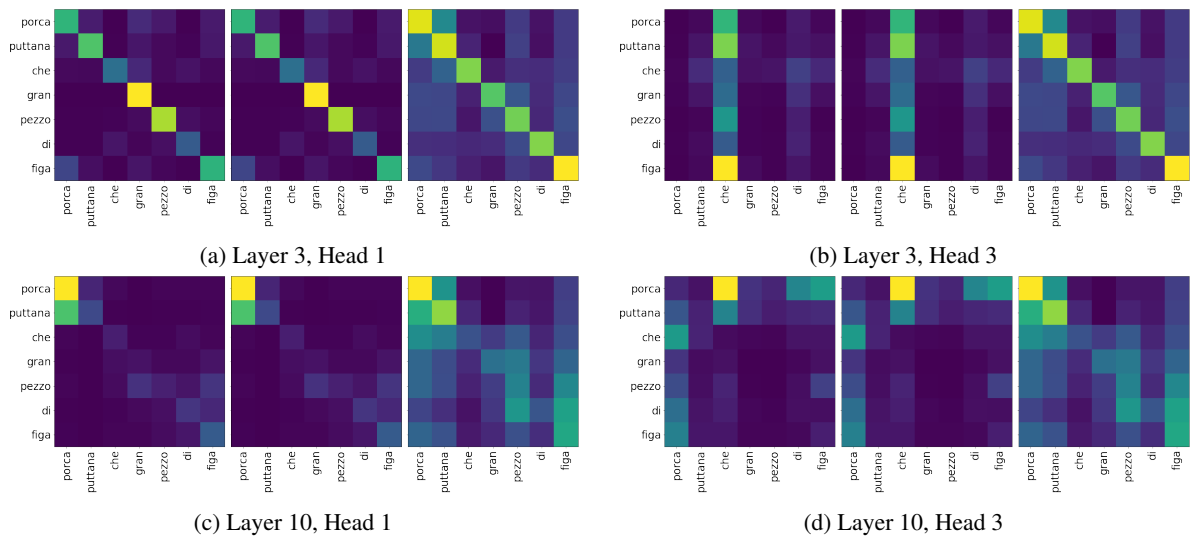
Figure 2: Attention (left), Effective Attention (center), and Hidden Token Attribution (right) maps at different layers in fine-tuned BERT. Lighter colors indicate higher weights. Sentence: “p*rca p*ttana che gran pezzo di f*ga”, non-literal translation: “ holy sh*t what a nice piece of *ss ”.
