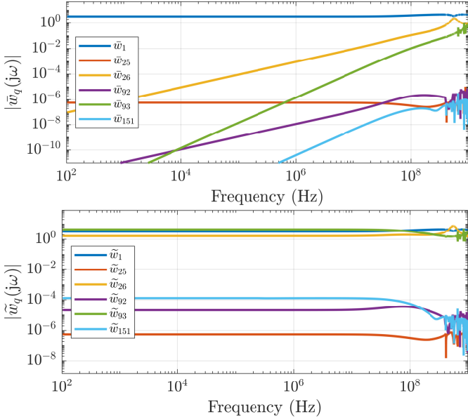
Fig. 10. Top panel: subset of basis functions obtained with the proposed Block-Diagonal SVD (BD-SVD); bottom panel: the same rescaled basis functions via (43).
