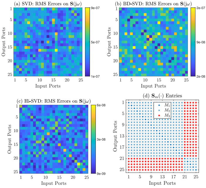
Fig. 9. Data compression applied to a 25-port shielding enclosure. Accuracy on all transfer function elements after compression via the Standard SVD (a) and the proposed Block-Diagonal SVD (b) and Hierarchical SVD (c). Panel (d) highlights the groups of responses according to the order of the DC zeros.
