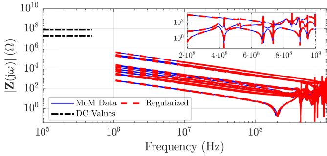
Fig. 5. Selected responses of regularized impedance parameters of a 5 \times 5 box ( P = 25 ) via Algorithm 1 ( R = 100 \text{ M}\Omega , r = 0.1 \text{ }\Omega ). Black dotted lines represent the DC values from (1); the inset provides a detail on high-frequency.
