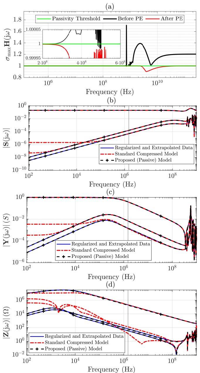
Fig. 13. As in Fig. 11, but for a 100-port shielding enclosure.
