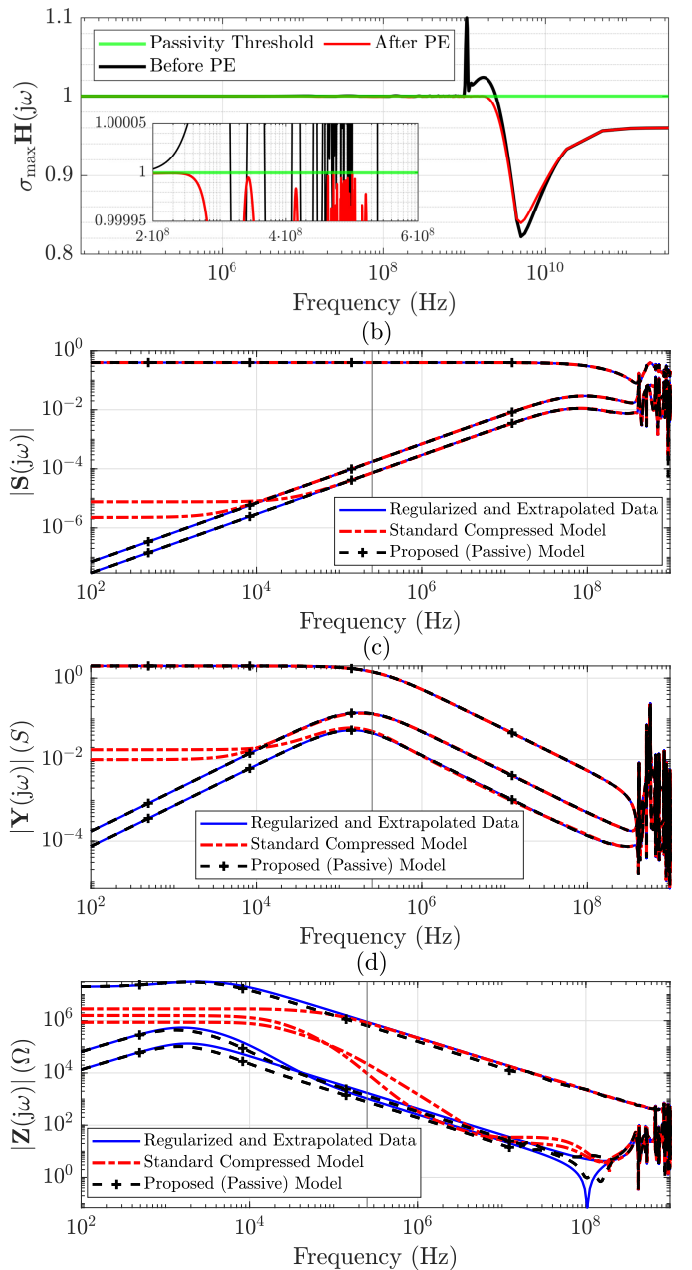
Fig. 11. Modeling a 25-port shielding enclosure: (a) envelop of the maximum singular values of scattering model responses before and after Passivity Enforcement (PE); (b)-(d) validation of standard and proposed macromodel responses in scattering, admittance and impedance representation.
