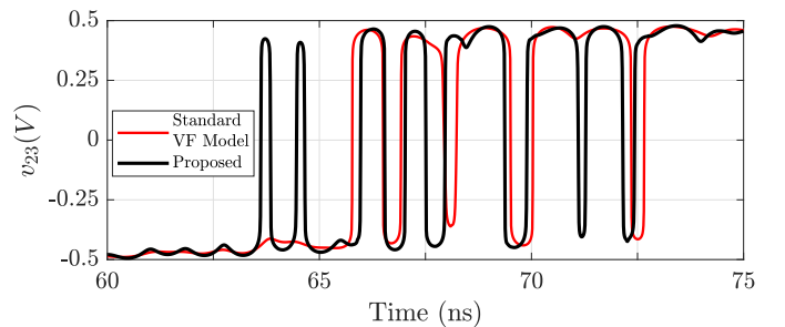
Fig. 12. Transient simulation of proposed model compared to a standard VF model. The excitation field is a double exponential (HEMP) waveform [32] defined as \mathcal{E}_{\text{inc}} = E_0(e^{-at} - e^{-bt})u(t) with a = 40 \times 10^6 \text{ s}^{-1} , b = 476 \times 10^6 \text{ s}^{-1} and amplitude E_0 = 50 \text{ kV/m} .
