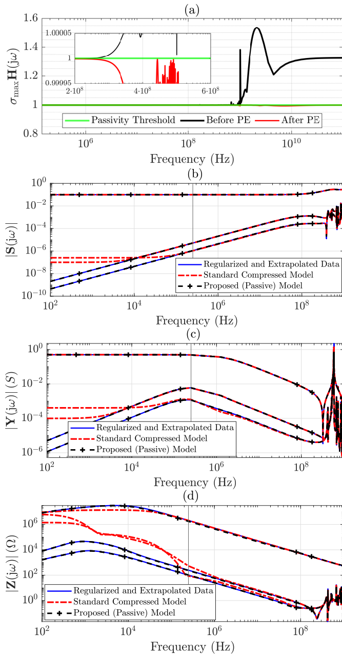
Fig. 14. As in Fig. 11, but for a 400-port shielding enclosure.
