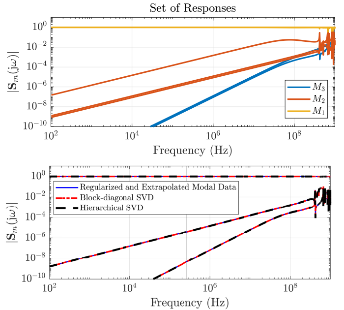
Fig. 8. Grouping responses of a 25-port box according to the order of DC zeros. Top: magnitude of the modal responses. Bottom: examples of responses with DC zeros which are recovered after proposed data compression approaches.
