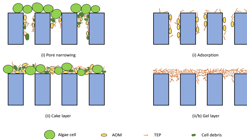
175 Fig. 1: Mechanisms of membrane fouling in membrane processes for biomass harvesting: (i) pore narrowing usually occurs 176 first, due the action of compounds (algal organic matter (AOM), transparent exopolymer particles (TEP) and cell debris) 177 smaller than membrane pores. Pore narrowing is enhanced by the simultaneous adsorption effect (i) related mainly to 178 biopolymers, i.e., AOM and TEPs. Cake layers are instead associated to larger particles, such as algal cells, which are less likely 179 to penetrate into the membrane pores and more prone to give rise to the so-called dynamic membrane. A gel-layer structure 180 (ii/b) is formed when biopolymers and bacteria are more present than algal cells in the feed stream.
