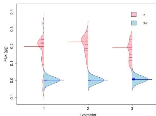
Figure 6: The three lysimeters containing the three soils studied (left); Phosphate fluxes measured at the inlet and outlet of the three lysimeters (right)
