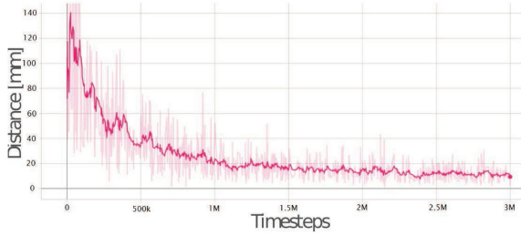
Fig. 5. Tracking error during the training.
