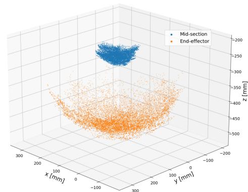
Fig. 2. AM-I-Support's task space.
