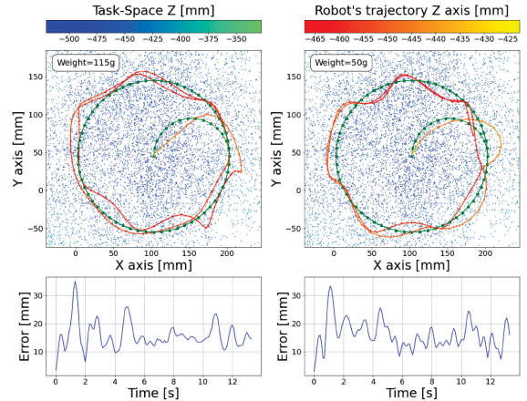
Fig. 8. Closed-loop trajectories on the AM-I-Support, with weights. The green target trajectory has an initial height that varies with the weight, and a final height of z = -460 mm.
