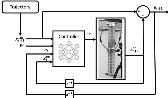
Fig. 6. Overview of the controlled system. z^{-1} represents a time delay operator.
