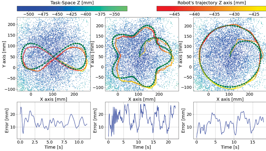
Fig. 7. Closed-loop trajectories and cartesian error on the AM-I-Support, without weights. The scattered green points indicate the target positions. The trajectory starts in the robot’s resting position ( z \approx -420 mm), and then move to a plane with z = -440 mm. During training, no planar trajectory was given as input, further proving the controller generalization capability.
