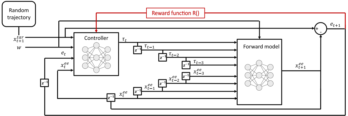
Fig. 4. Training Overview. The approximated forward model acting as an environment receives as inputs the current and past positions and actuations and predicts the next position. The controller acts as the RL agent, receiving the randomly generated target position, the weight carried, the current error, and the current position, and predicting the next optimal actuation to maximize the reward. z^{-1} represents a time delay operator.
