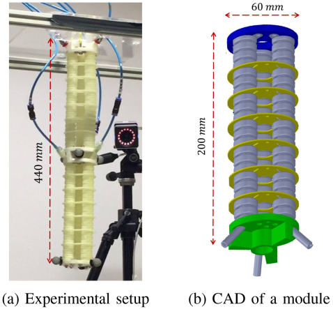
Fig. 1. AM-I-Support robot. Refer to [23] for further details.
