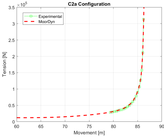
Fig. 4. Static Validation C2a
