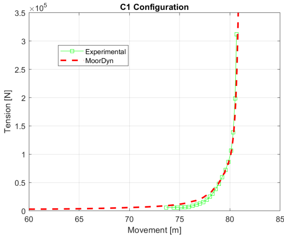
Fig. 5. Static Validation C1
