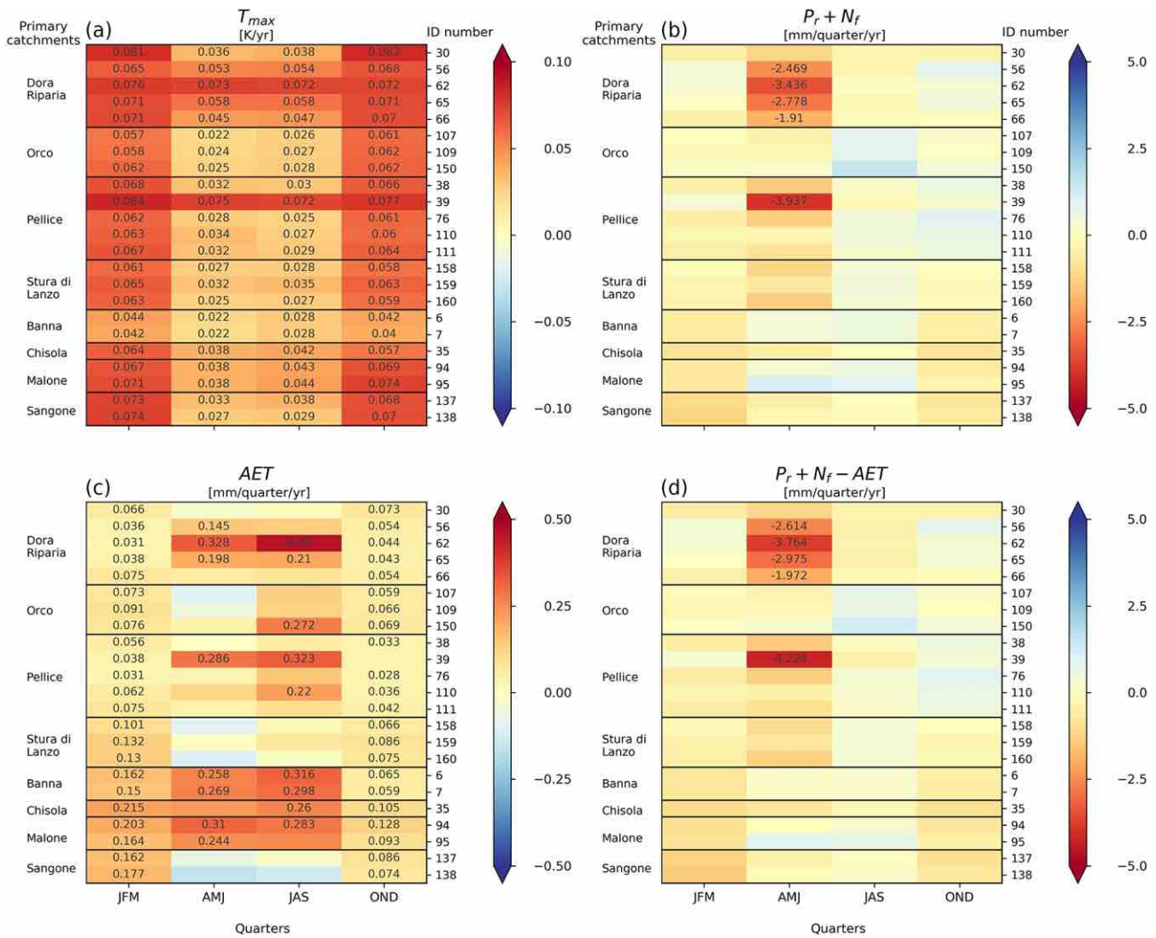
Figure 5. Trend slope of all quarters and catchments considered. (a) T_{max} , (b) precipitation, (c) AET and (d) drainage. Trend slope is specified if significant at a 5% level. When quarters are considered, the precipitation is represented by the sum of liquid precipitation P_r and melted snow N_f .
