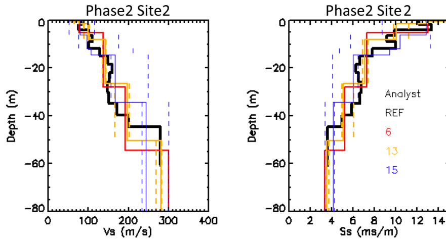
Fig. 10 Phase 2 site 2. Interpretation of layering from micro-tremor array method (MAM) models based on sparse array (triangle) of geophones. Left: the horizontal axis is shear-wave velocity V_S . Right: the horizontal axis is slowness S_S (inverse
