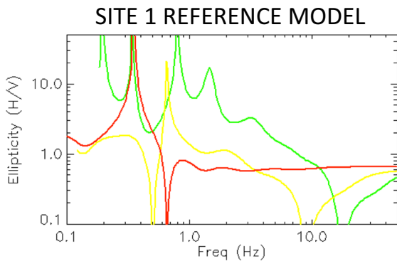
Fig. 16 Rayleigh wave ellipticity curves for site 1, modeled using the reference model of Figs. 2a and 3. Red, yellow, and green colors show fundamental ( R_0 ) and higher ( R_1 and R_2 ) modes, respectively
