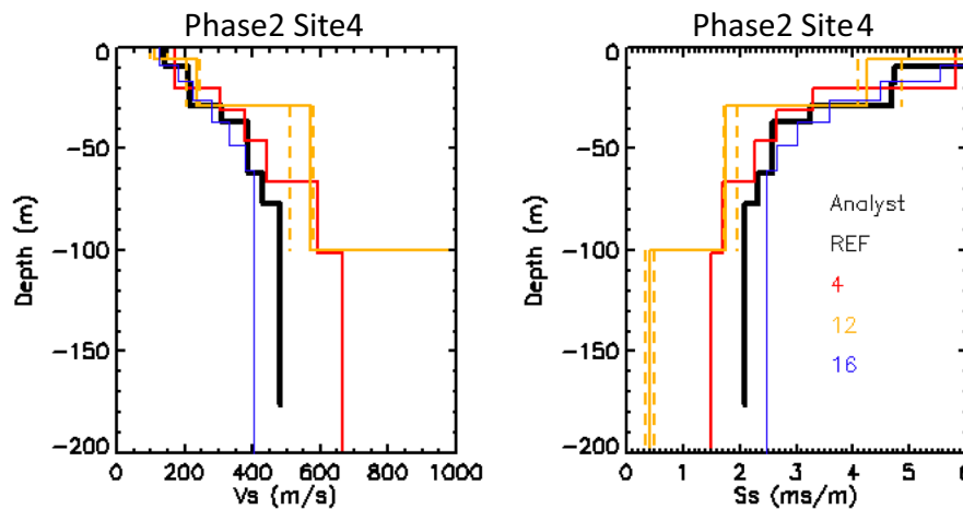
Fig. 11 Phase 2 site 4. Interpretation of layering from micro-tremor array method (MAM) models based on sparse array (nested triangles) of geophones. Left: the horizontal axis is shear-wave velocity V_S . Right: the horizontal axis is slowness S_S (inverse of V_S ). Black: the reference model supplied after all phases of blind interpretation. Red, yellow, and blue colors
