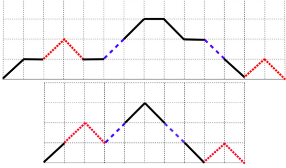
FIG. 5. (a) Example of a colored Motzkin path, with q = 3 colors, which corresponds to a particular Motzkin spin state |m_p^{(14)}\rangle = |\uparrow_1^1 0_2 \uparrow_3^2 \downarrow_4^2 0_5 \uparrow_6^3 \uparrow_7^1 0_8 \downarrow_9^1 0_{10} \downarrow_{11}^3 \downarrow_{12}^1 \uparrow_{13}^2 \downarrow_{14}^2\rangle . (b) Example of a colored Dyck path which corresponds to a particular Dyck spin state |d_p^{(10)}\rangle = |\uparrow_1^1 \uparrow_2^2 \downarrow_3^2 \uparrow_4^3 \uparrow_5^1 \downarrow_6^1 \downarrow_7^3 \downarrow_8^1 \uparrow_9^2 \downarrow_{10}^2\rangle .
