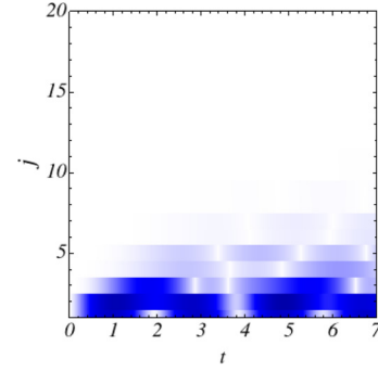
FIG. 8. Time evolution of \langle S_z(j, t) \rangle - \langle S_z(j, 0) \rangle , for the dimerized-frustrated model [30] (with \delta = 0.8 and \alpha = 0 following the notation in Ref. [30]), after switching on a local field, 5S_z(j_0) , at j_0 = 0 .
