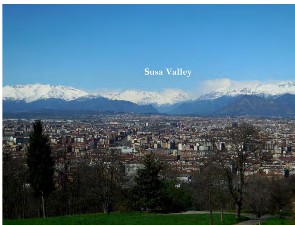
Fig. 2 - Gently eastward sloping morphology of Turin, which has been built on the wide outwash fan supplied by the Susa Valley, drained by the Dora Riparia River, as seen from Turin Hill.
