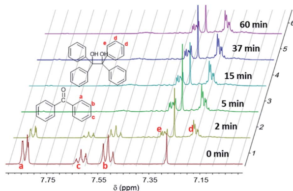
Fig. 2 1 H NMR spectra of formulation (A + B) at 0, 2, 5, 15, 37 and 60 min of UV irradiation.
