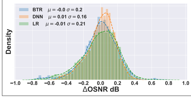
Figure 6: Probability density functions of \Delta\text{OSNR} for all ports of the 8x8 Beneš switch, using BTR, LR, and DNN.
