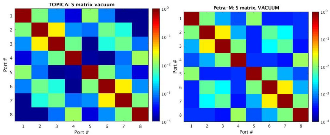
Figure 3. Comparison of the absolute value of the S-matrix (8 x 8) elements for the vacuum case between TOPICA (left figure) and Petra-M (right figure).
