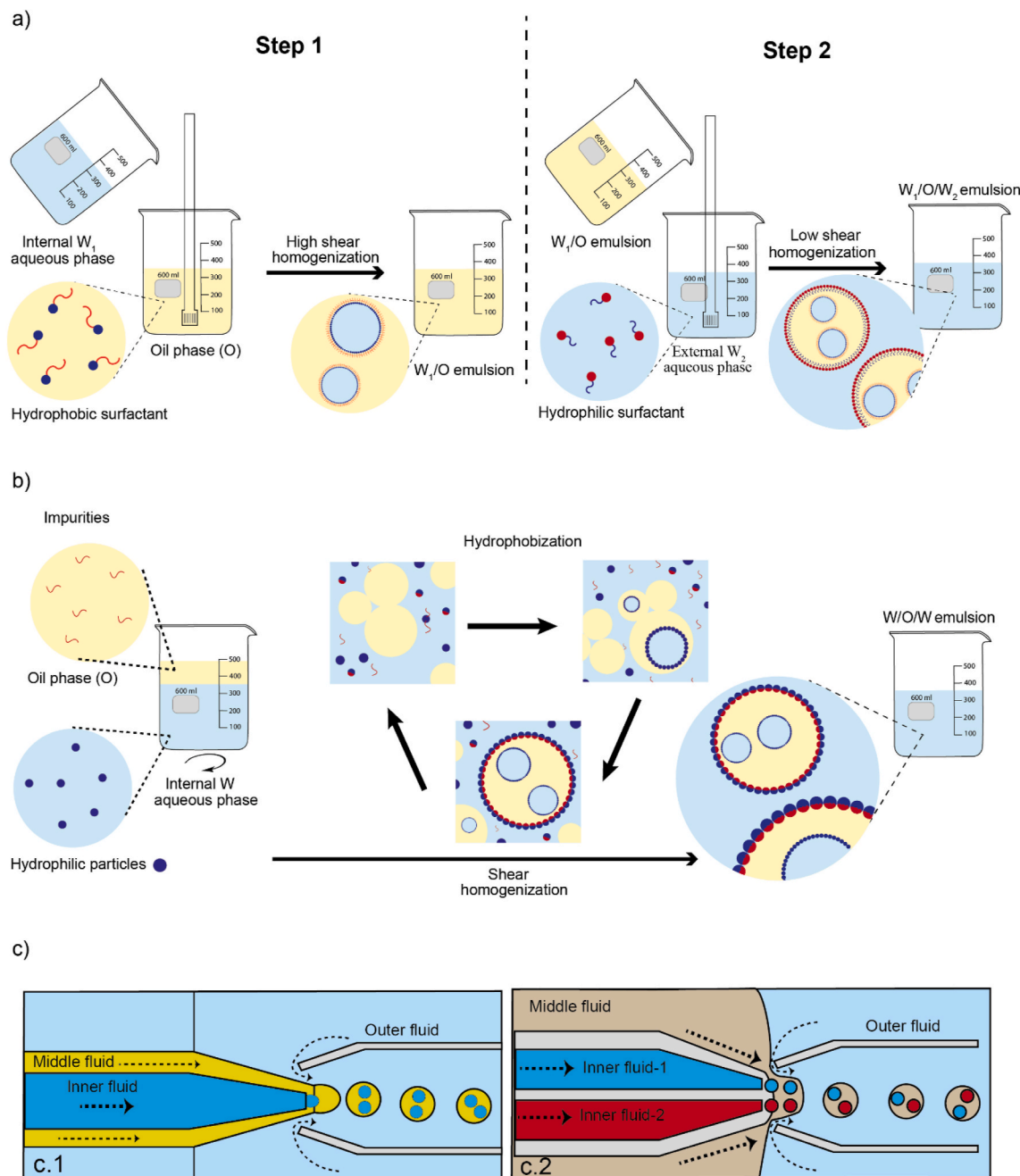
Fig. 1. Schematic presentation of different methodologies used to prepare DEs: a) two-step emulsification used for surfactant-stabilized DEs, b) one-step emulsification used for particle-stabilized DEs and c) microfluidic device used to prepare DEs (1) and DEs with different composition in the inner aqueous phase (2). Figure c) adapted from Adams et al. (2012).
