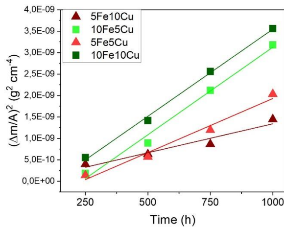
Figure 9: Parabolic rate plot with linear trend lines of coated Crofer 22 APU during cyclic oxidation at 750 °C in air (250–1000 h).
