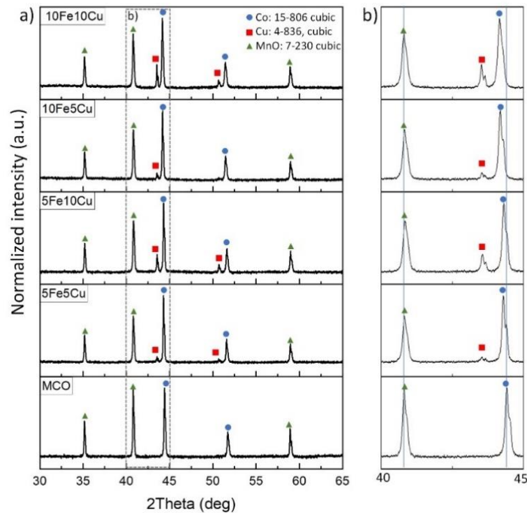
Figure 2: X-Ray diffraction patterns of the Fe and Cu doped coatings and pristine MCO after the reducing heat treatment. Patterns are normalized to the intensity of the highest peak. (b) Excerpt of patterns between 40° and 45°.
