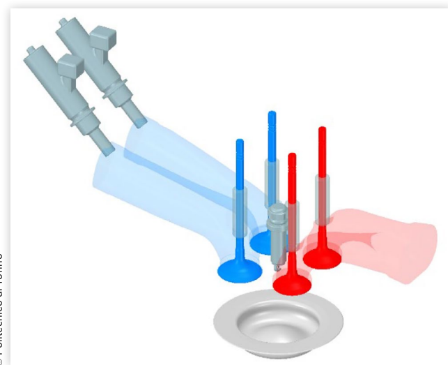
FIGURE 1 Selected architecture for combustion system conversion from diesel to H 2 engine.
