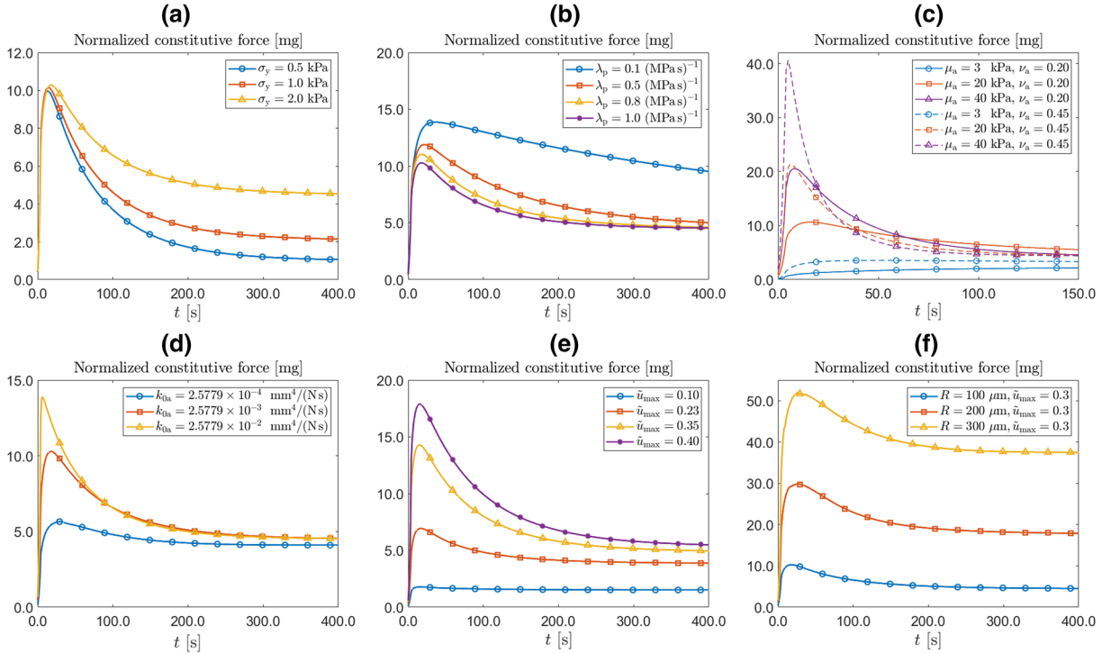
FIG. 8. Relaxation curves for the constitutive exchanged force obtained for various values of the parameters \sigma_\gamma , \lambda_p , \mu and \nu , k_{0a} , \tilde{u}_{\text{max}} = u_{\text{max}}/(2R) and R . In these pictures, we took t_{\text{ramp}} = 5 s and t_{\text{end}} = 405 s. These curves are obtained by integrating the function -\left[\sigma_a^{(\text{sc})}\right]^{zz} over the contact surface \Sigma_u(t) of the aggregate with the upper plate. The parameters that are not changed are reported in Table 1. Note that, also in this case, all the curves plotted in this figure refer to the case with remodelling
