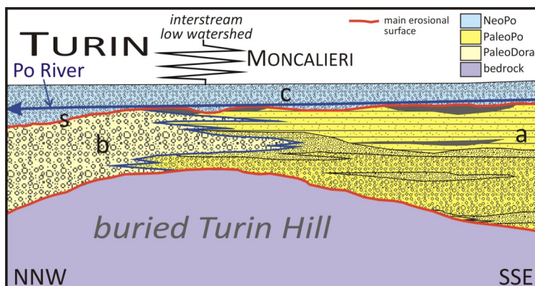
Fig. 8 - The alternating gravel and fine-grained sediments with peaty layers (black) deposited by the paleo Po River ( a ) during the Upper Pleistocene suggest the formation of marshes in the plain south of Turin. The gravel deposited by the paleo Dora River ( b ) indicates the aggradation of the Dora Riparia outwash fan. A low watershed developed between the two areas, currently buried. Subsequently, the shaping of an evident erosional surface ( s ) and the neo Po sediments ( c ) deposited in the late Upper Pleistocene indicate the formation of the current Po River through an outwash phenomenon.
