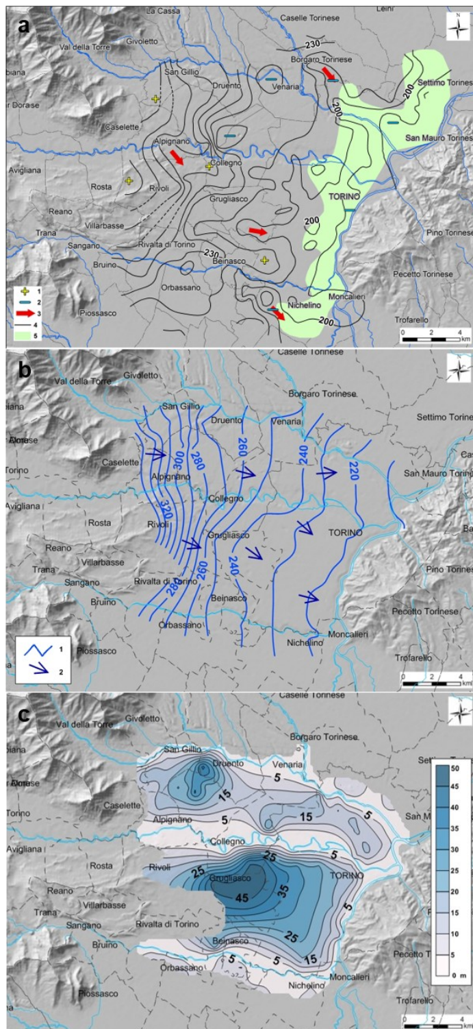
Fig. 22 - a) Map of the base of the outwash and fluvial Complex (1-highest altitude zones; 2-lowest altitude zone; 3- paleochannels; 4- contour lines of the Complex base in a.s.l. m; 5- buried erosional surface); b) Piezometric map of the shallow unconfined aquifer (January 2000) (1-isopiezometric lines in a.s.l. m; 2-flow lines); c) Map of depths to the groundwater table (January 2000).
