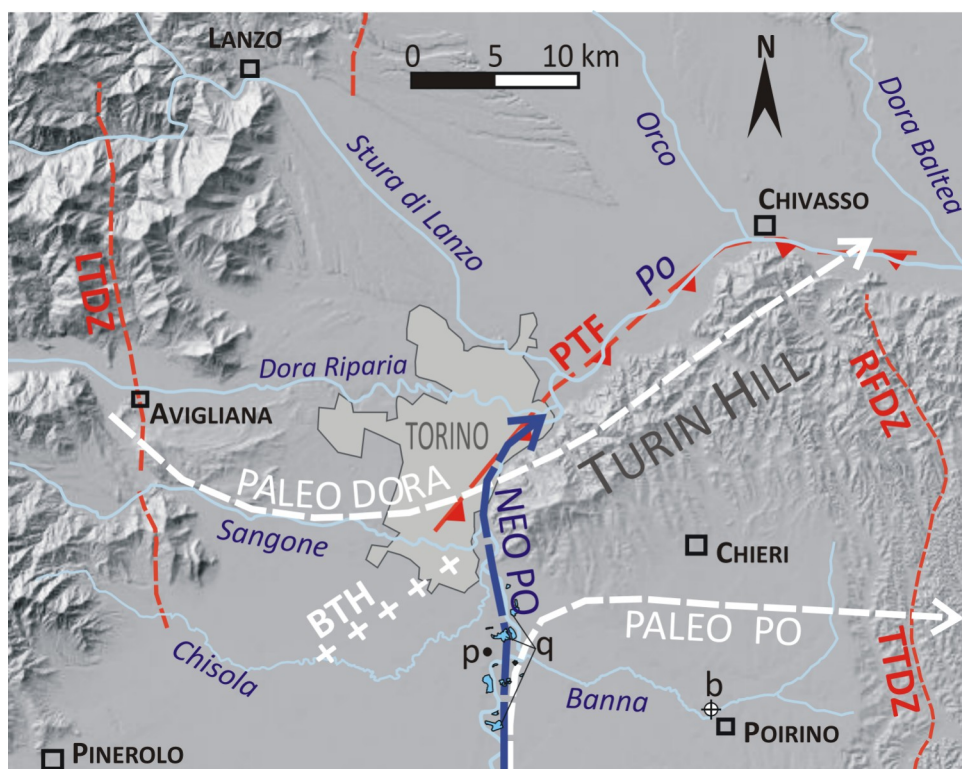
Fig. 7 - The fluvial succession mapped in Turin Hill proves that in the Upper Pleistocene the hydrographic pattern was formed by a paleo Dora River, that flowed on the western and northwestern slopes of Turin Hill, and a paleo Po River that flowed through its southern side (white arrows). The neo Po River develops during the late Upper Pleistocene, through an overflow phenomenon, flowing toward north (blue arrow). BTH: Buried Turin Hill; PTF: Padane Thrust Front; TTDZ: T. Traversola Deformation Zone; RFDZ: Rio Freddo Deformation Zone; LTDZ: Colle del Lys-Trana Deformation Zone. The peaty sediments connected to the paleo Po River and described in the Moncalieri-La Loggia quarries by Tropeano (1987) (q), observed in an ancient outcrop at la Loggia (p) (Fig. 9) and drilled in a recent borehole at Poirino (b) (Fig. 10) are also reported.
