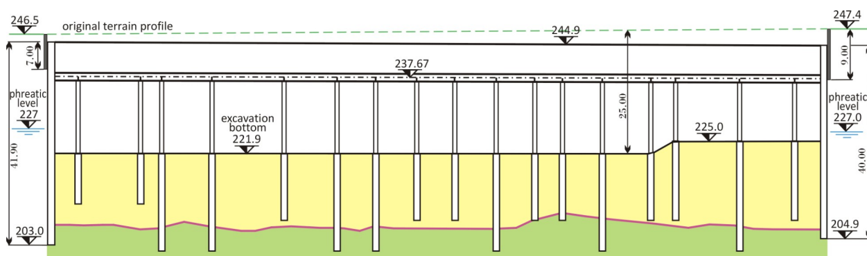
Fig. 16 - Cross section of the excavation of the Intesa Sanpaolo skyscraper (S in Fig. 14) essentially involving the outwash sandy gravelly sediments (yellow), with a boulder level, that lie on the silty Villafranchian succession (green). Altitude is referred as m a.s.l.
