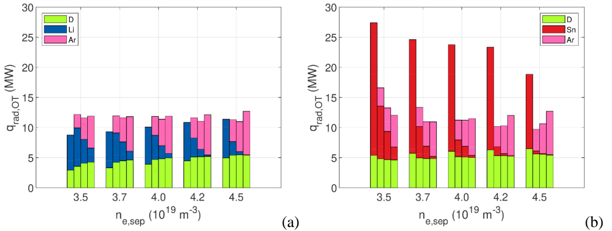
Figure 20. Contributions to the radiated power density, integrated over the pedestal region, for Li (a) and Sn (b). For each value of n_{e,\text{sep}} , the four bars correspond to increasing Ar seeding levels, from \Gamma_{\text{Ar}} = 0 to \Gamma_{\text{Ar}} = 1 \cdot 10^{21} \text{ s}^{-1} . Note the different scales.
