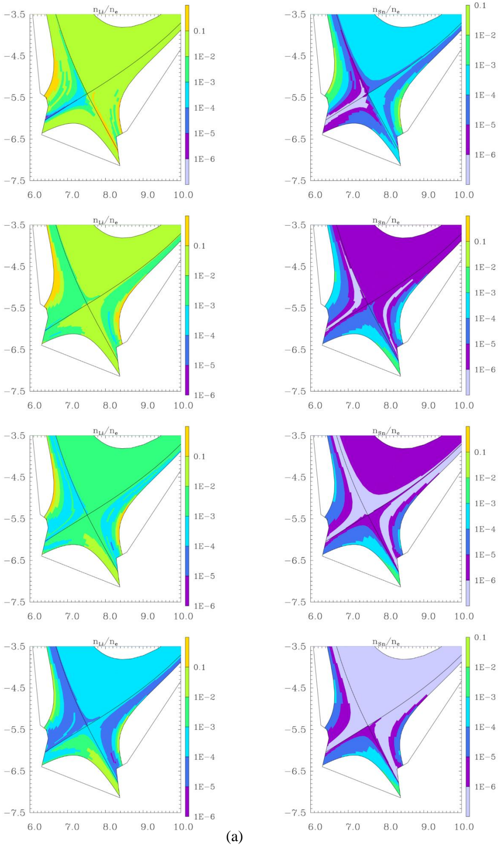
Figure 15. Computed 2D distributions of the relative concentrations n_{Li}/n_e (a) and n_{Sr}/n_e (b) in the edge plasma for the cases with n_{e,sep} = 4.5 \cdot 10^{19} \text{ m}^{-3} , for increasing Ar seeding rates (from \Gamma_{Ar} = 0 to \Gamma_{Ar} = 1 \cdot 10^{21} \text{ s}^{-1} , moving from top to bottom).
