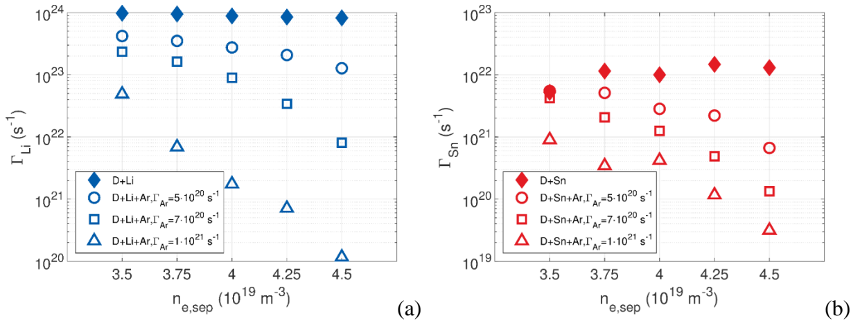
Figure 12. Total target erosion rate as a function of n_{e,sep} for the different Ar seeding rates considered in this work, for Li (a) and for Sn (b). Note the different y scale.
