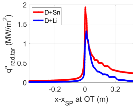
Figure 11. Outboard target profiles of radiation heat load computed for Li and Sn, for n_{e,sep} = 4.5 \cdot 10^{19} \text{ m}^{-3} .
