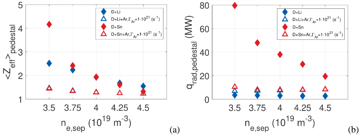
Figure 17. Average Z_{eff} in the pedestal region for different Ar seeding rates: comparison Li vs. Sn (a), and radiated power density integrated over the pedestal region for various Ar seeding rates: comparison Li vs. Sn (b). Only the cases with \Gamma_{Ar} = 0 and \Gamma_{Ar} = 1 \cdot 10^{21} \text{ s}^{-1} are shown, for clarity.
