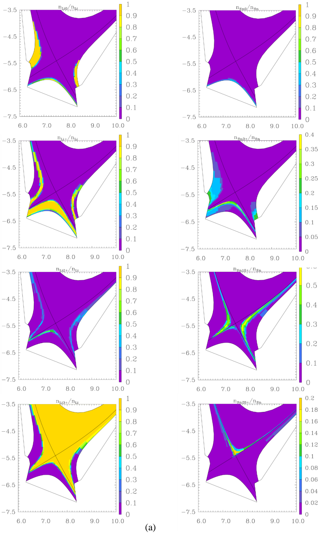
Figure 6. Computed 2D distributions of the relative abundance of Li^0 , Li^+ , Li^{2+} , Li^{3+} with respect of the total Li density (a) and of Sn^0 , Sn^{3+} , Sn^{10+} , Sn^{20+} with respect of the total Sn density (b) in the edge plasma for the
