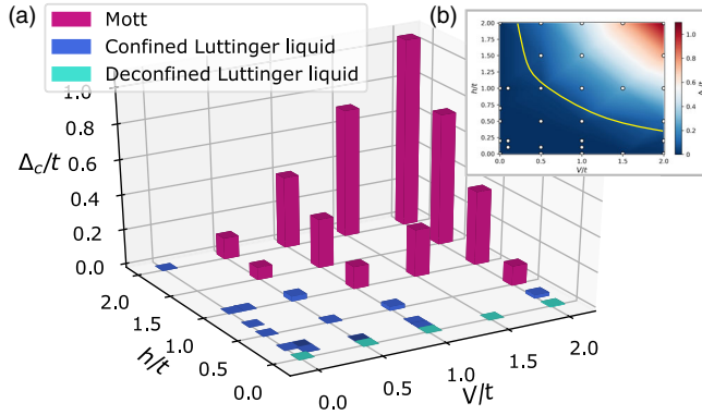
FIG. 2. Charge gap extrapolated in the thermodynamic limit, \Delta_c , at filling n^a = 2/3 as a function of h and V . (a) As a guide for the eye the violet (blue) bars denote \Delta_c/t > 0.05 ( \Delta_c/t \leq 0.05 ) where we expect a Mott insulator (Luttinger liquid). (b) Heatmap of the gap diagram where the yellow curve, added by hand, corresponds to the approximate phase boundary.
