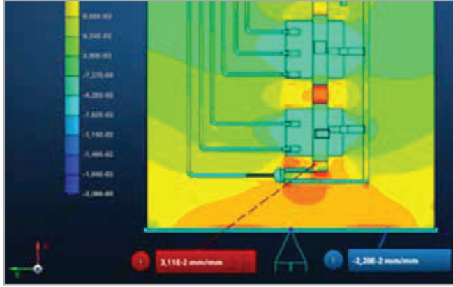
Fig. 4 – \epsilon_{xx}=0.0311 at the downward imposed displacement
