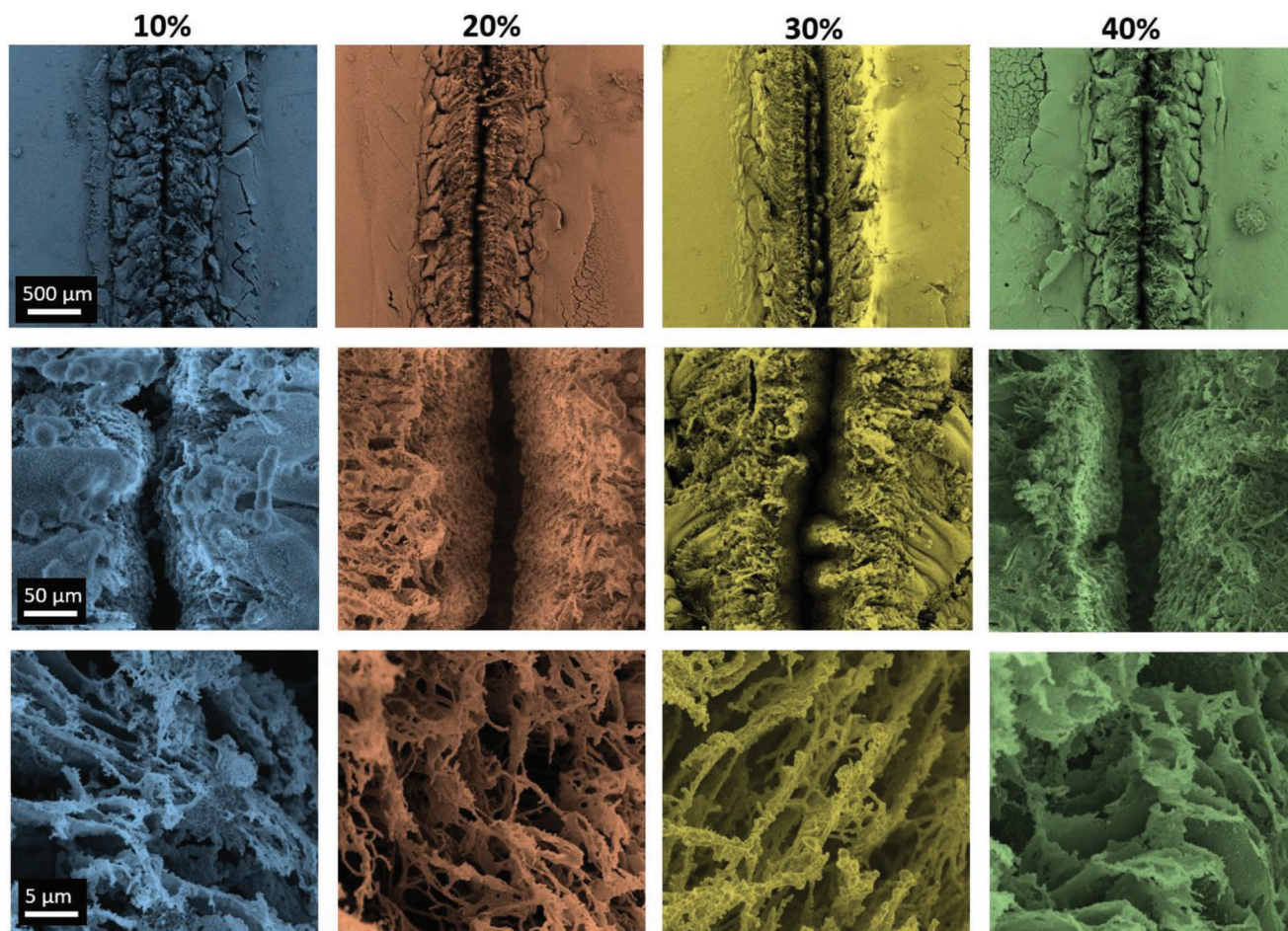
Figure 2. FESEM images at different magnifications (increasing from top to bottom) of the LIG samples obtained from PDMS treated with different concentrations of TEG (10%, 20%, 30%, and 40%).
