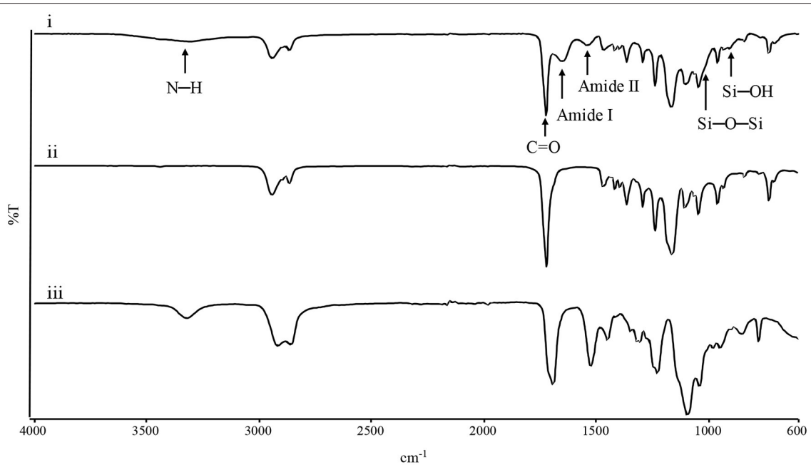
FIGURE 2 | ATR-FTIR spectra of (i) PCL-Gel, (ii) PCL, and (iii) Gel membranes.
