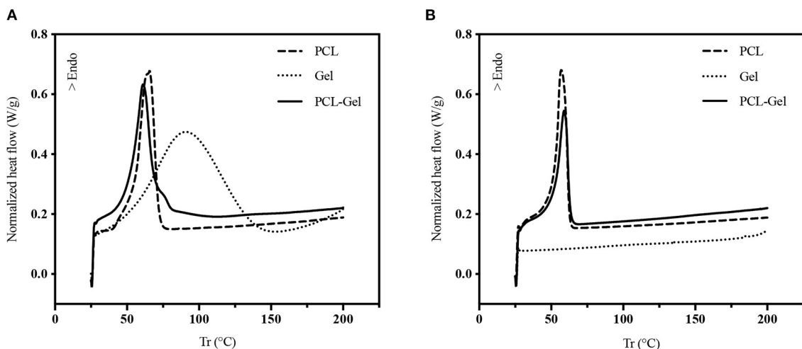
FIGURE 3 | DSC thermogram of the (A) 1st and (B) 2nd heating cycle (10°C/min) of PCL, Gel, and PCL-Gel membranes.
