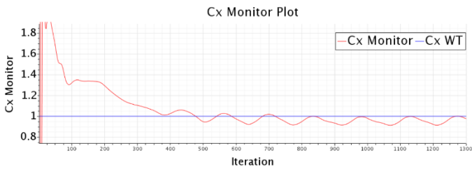
Figure 17 Standard configuration. C_x trend normalized to wind tunnel value
