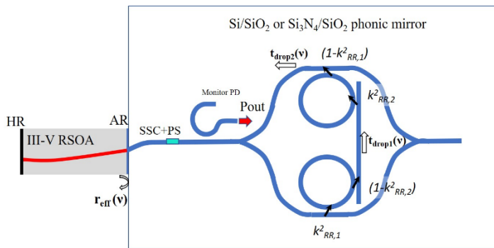
Figure 1: Sketch of the hybrid external-cavity laser structure. The mirror is based on a Mach Zehnder Interferometer (MZI) loaded by two rings providing a narrowband complex reflectivity r_{\text{eff}}(v) and a Vernier tuning of about 150 nm. The symbols are: PS = phase control sections, k_{RR,1,2}^2 = power coupling coefficient of the two ring resonators in the critical coupling configuration ( k_{RR,1,2} ), t_{\text{drop},1,2} = drop port transmission coefficients of the two ring resonators, SSC = spot size converter. The output power P_{\text{out}} is collected by the coupler with output coupling coefficient T_{c,\text{out}} .
