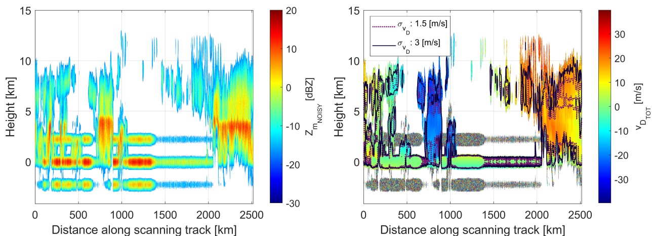
Figure 14. Reflectivities and Doppler results corresponding to a full revolution of the WIVERN antenna as shown in Fig. 12 for an integration length of 1.0 km ( M=8 ). Left panel: simulations of the WIVERN reflectivities (signal+noise) with ghost echoes at 2.3 km above and below the ground due to the depolarisation by the surface leading to ghost echoes where there is no real cloud. Right panel: WIVERN retrieved line-of-sight Doppler velocities after performing the polarization diversity pulse pair processing. continuous (dashed) black contour lines correspond to Doppler velocity precision of 3 (1.5) m/s according to Eq. (15)). Note that the ghost echoes have lower precision.
