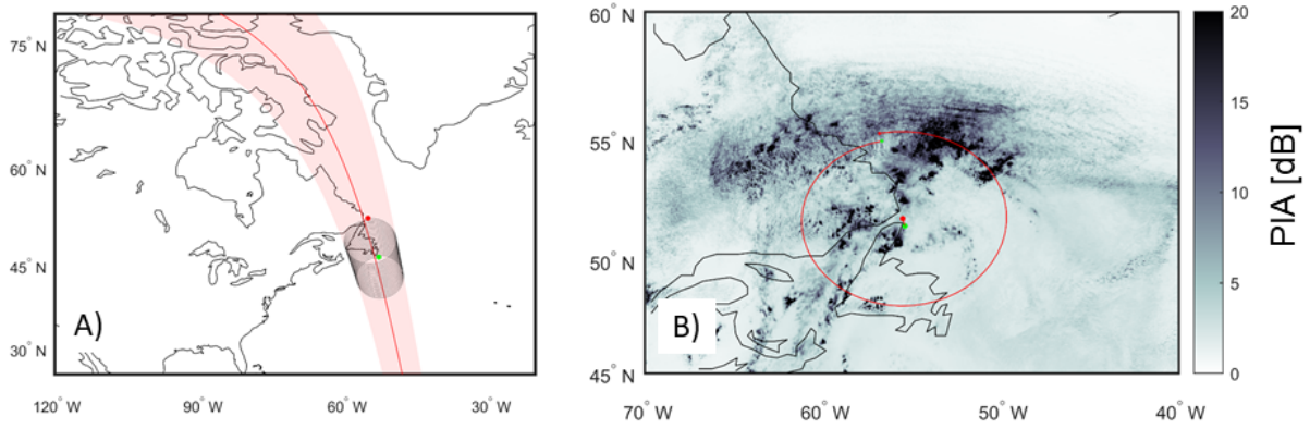
Figure 8. Panel A: WIVERN satellite track off the Labrador coast with the satellite ground track (red line), the scanning swath (shaded red region) and the radar footprints (black line) for 20 full revolutions of the conically scanning antenna corresponding to a flight time of 100 s. Panel B: details of a single revolution of the WIVERN antenna. This rotation sample will be examined in detail later (see Figs. 11-14).
