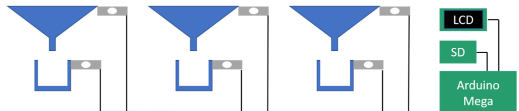
Figure 6. Scheme of the apparatus used for the test.
