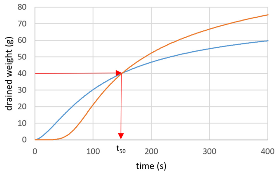
Figure 5. Two different foam decay processes (one described by the blue line and the other by the orange one) that exhibit the same half-life time.
