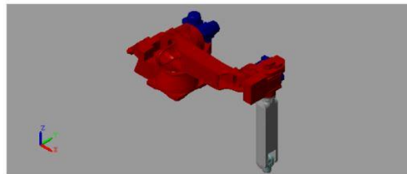
Figure 4. Kinematic simulation of the Comau Smart SiX 6-1.4: (a) robotics toolbox (b) Simscape.
