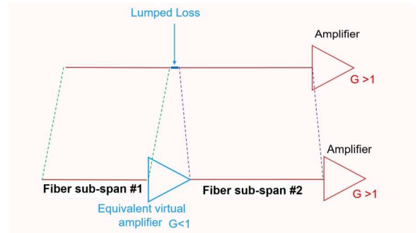
Fig. 1: Split-span model for lumped loss.
