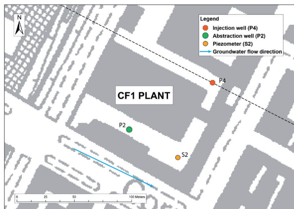
Fig. 3b - Politecnico CF1 plant GWHP System overview. P2 abstraction well. P4 - reinjection well. S2 - control piezometer. Dotted line indicates the direction of the cross-section line reported in Figure 1 (Modified from Gizzi et alii, 2020)
