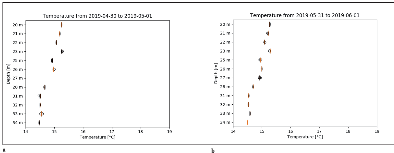
Fig. 6 - Boxplot diagrams of different spring season plant-operation times: a. 01/05/2019; b. 01/06/2019. Data recorded by the water temperature measuring chain installed in piezometer (S2)
