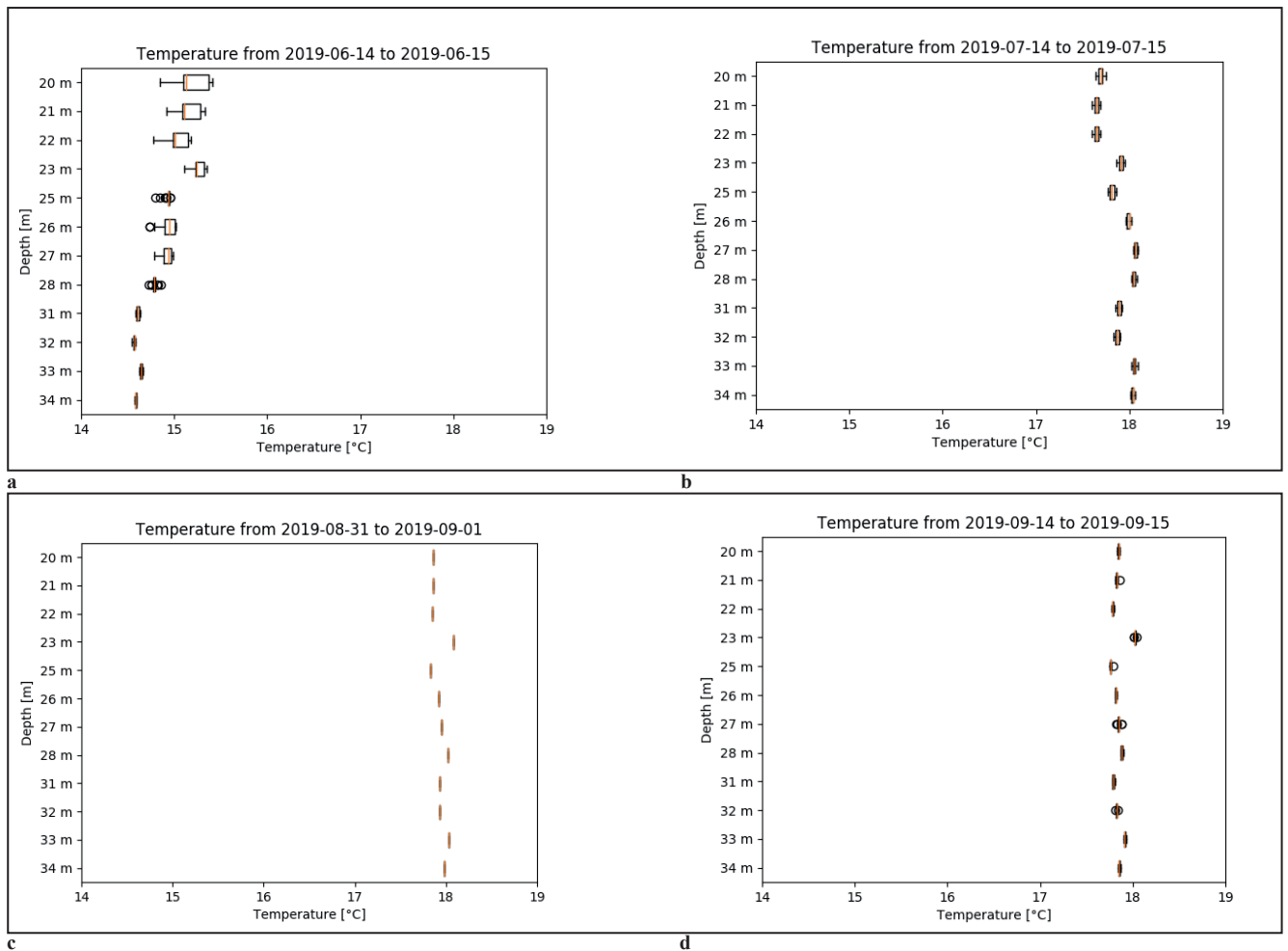
Fig. 7 - Boxplot diagrams of different summer season plant-operation times: a. 15/06/2019; b. 15/07/2019; c. 01/09/2019; d. 15/09/2019. Data recorded by the water temperature measuring chain installed in piezometer (S2)
