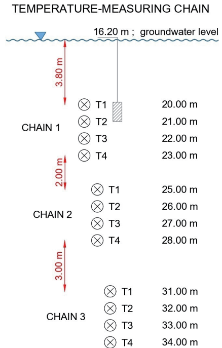
Fig. 4 - Simplified conceptual scheme of the water temperature measuring chain (PT1004/Pt) installed in S2-control piezometer of the Politecnico of Torino open-loop GWHPs
