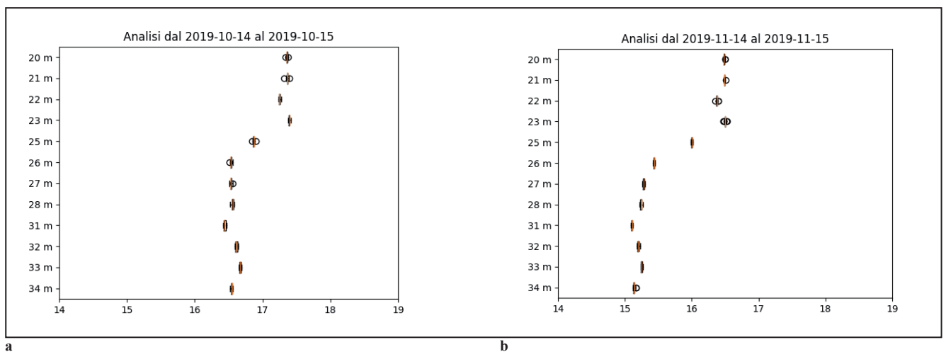
Fig. 8 - Boxplot diagrams of different autumn season plant-operation times: a. 15/10/2019; b. 15/11/2019. Data recorded by the water temperature measuring chain installed in piezometer (S2)
