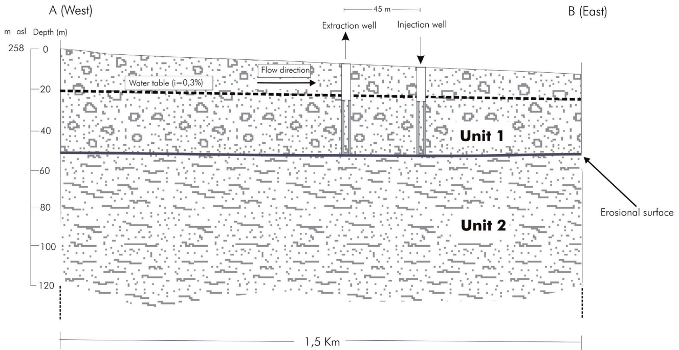
Fig. 2 - Schematic hydrogeological cross-section of the study area (modified from Lo Russo et alii, 2018)
