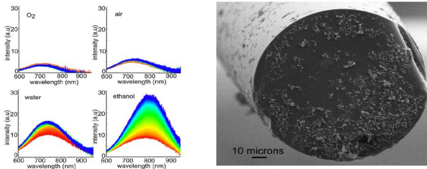
Fig. 15. a) Fluorescence spectra of the Si-QDs exposed to oxygen, air, water vapor, and ethanol vapor over 1h. b) SEM image showing Si-QDs at the end of an OF. Reproduced from [67]. Copyright 2013, with permission from Elsevier.
