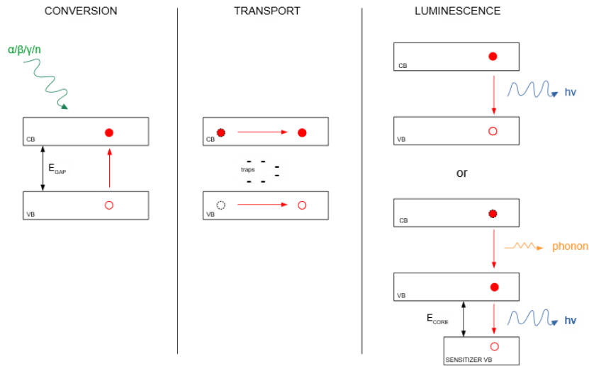
Fig. 1. Schematization of the three steps involved in the scintillation process.
