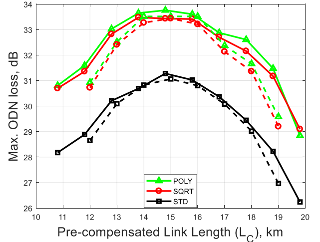
Fig. 7. Maximum ODN loss as a function of L_C , with the optimum V_{pp} of driving signal. Solid: experiments with L=15.8 km and P_{TX}=11 dBm. Dashed: simulations with L=16.0 km and P_{TX}=11 dBm (dashed curves extracted from Fig.4).
