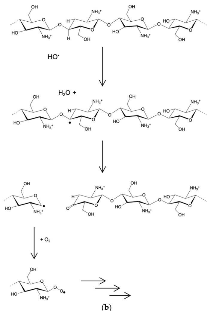
Scheme 2. Sketch representing the decrease in length for immobilised chitosan chains subject to attacks by \text{HO}^\bullet radicals (a) and example of a possible chain scission mechanism in the aerated aqueous solution used for grafting (b).
