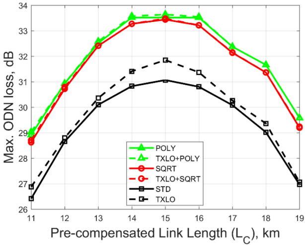
Fig. 4. Maximum ODN loss as a function of L_C , for L = 16 km and P_{TX} = 11 dBm, with the optimum V_{pp} of driving signal. Solid: without TXLO, dashed: with TXLO.
