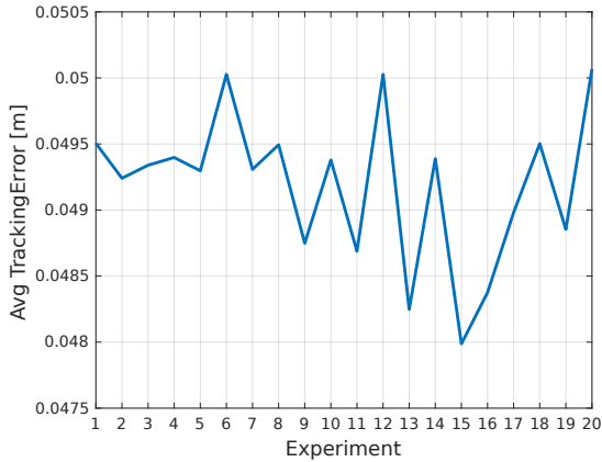
Fig. 6 The average tracking error for 20 trajectories running the same scenario of Figure 4.
