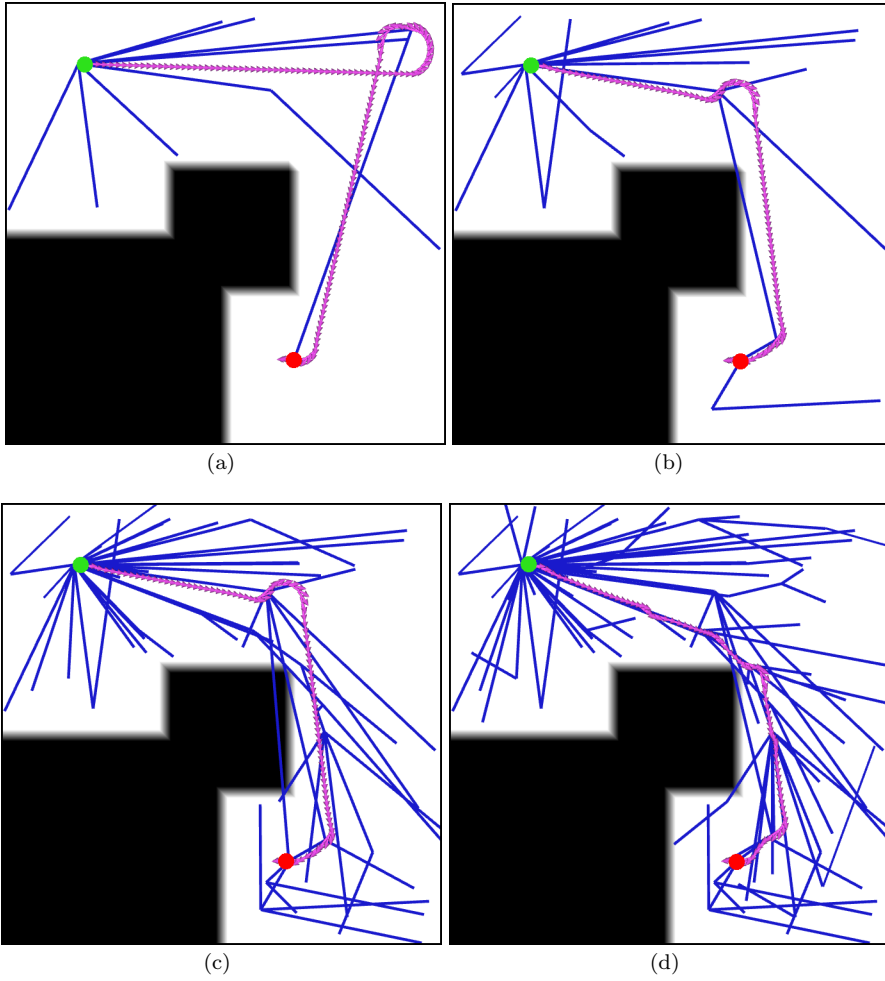
Fig. 4 The construction of the exploration tree using the MP-RRT # algorithm. The start and target positions are in green and in red, respectively. The graph \mathcal{G}^Y in the reference space is colored in blue, while the computed path obtained from the graph \mathcal{G}^X in the state space is colored in magenta. In (a), the graph consists of 10 vertices rooted from the start pose finding an initial solution in the map with a cost (i.e. the path length) of 66.44 m. In (b), the graph with 20 vertices, in which the solution is improved with a cost of 45.09 m. In (c), the graph consists of 60 vertices, but the solution is not improved. In (d), the graph has 100 vertices obtaining a solution with cost 38.70 m.
