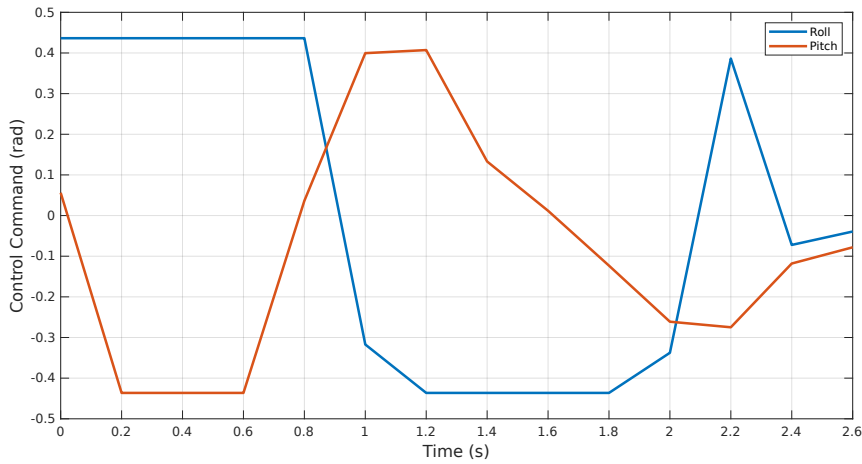
Fig. 3 The roll and pitch control inputs computed by MPC to follow the trajectory of Figure 2.
