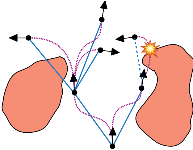
Fig. 1 Example of graphs constructed with MP-RRT#. The graph \mathcal{G}^{\mathcal{Y}} consists of vertices (in black) and edges (in blue) in the reference state. Instead, the graph \mathcal{G}^{\mathcal{X}} consists of trajectories (in magenta) obtained through evaluating the edges of \mathcal{G}^{\mathcal{Y}} using the MPC strategy. An edge of \mathcal{G}^{\mathcal{Y}} is labeled as invalid if its corresponding trajectory in \mathcal{G}^{\mathcal{X}} crosses an obstacle.
