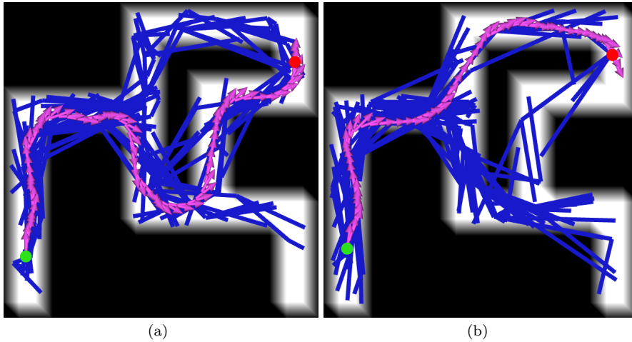
Fig. 7 Trajectories computed with the MP-RRT # by constructing a graph with 400 vertices. The start and target positions are in green and in red, respectively. In blue, the graph \mathcal{G}^Y in the reference space, while in magenta, the computed path obtained from the graph \mathcal{G}^X in the state space. In (a) and (b) the target is in a similar position, but with opposite orientation. As a consequence, the solution is completely different, yielding different paths.
