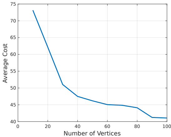
Fig. 5 The average cost of the solution path against the number of vertices in the MP-RRT # algorithm. The average cost is computed running the algorithm 50 times in the same scenario of Figure 4.
