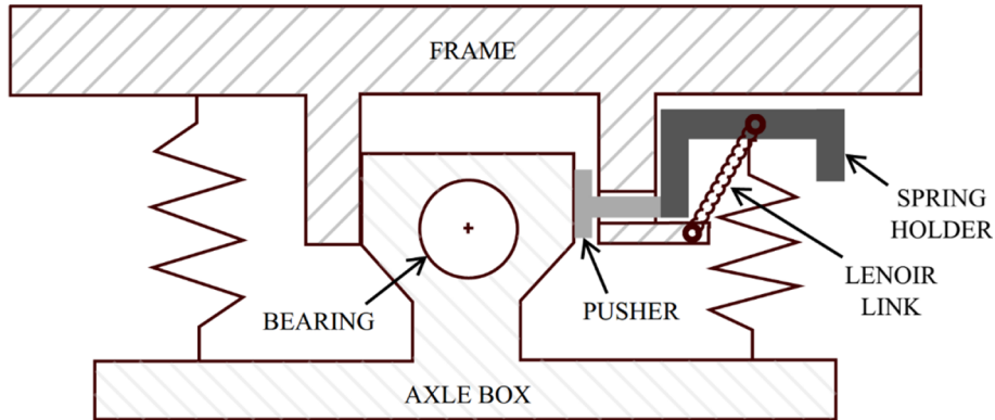
Fig. 4 Lenoir link mechanism
