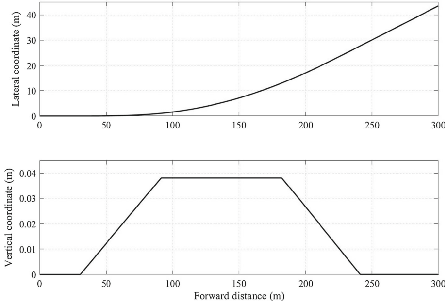
Fig. 10 Track geometry
