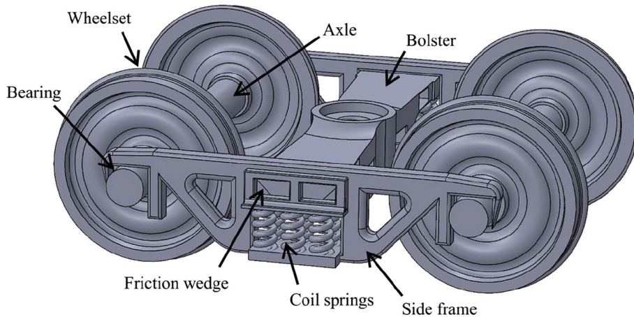
Fig. 1 Three-piece bogie
