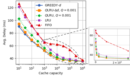
Fig. 5. Comparison of online policies and GREEDY- d : average delay versus cache capacity.
