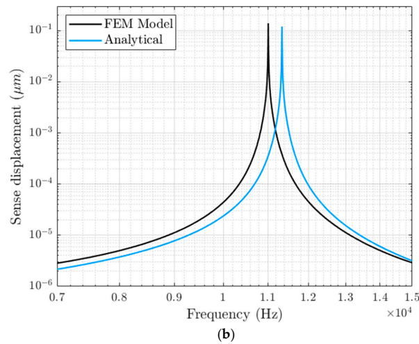
Figure 10. Comparison between the FEM-based and analytical frequency response amplitude in the sense direction for the proposed dual mass MEMS gyroscope (logarithmic scale), obtained with 50 V DC and 5 V AC actuation voltage and \Omega_z = 300^\circ/s , (a) without electrostatic tuning, (b) with electrostatic tuning.
