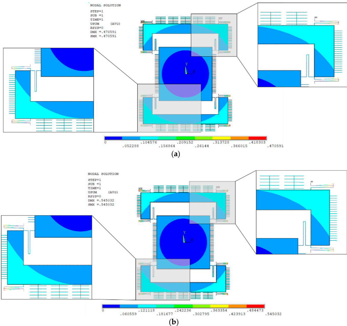
Figure 12. Structural thermal deformation in the proposed dual mass MEMS gyroscope (a) at -40\text{ }^\circ\text{C} , (b) at 100\text{ }^\circ\text{C} , with reference temperature T_F of 25\text{ }^\circ\text{C} .
